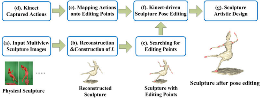
Fig. 4. Proposed platform for assisting sculpture design: (a) inputting a set of multi-view sculpture images, (b) reconstructing a virtual 3D sculpture and calculating its Laplace operator L , (c) searching for candidate editing points on the surface of the sculpture, (d) using Kinect to capture body actions of the sculptor, (e) mapping body actions onto the surface of the sculpture by a pre-defined configuration set, (f) Kinect-driven sculpture pose editing, and (g) obtaining pose editing results.
